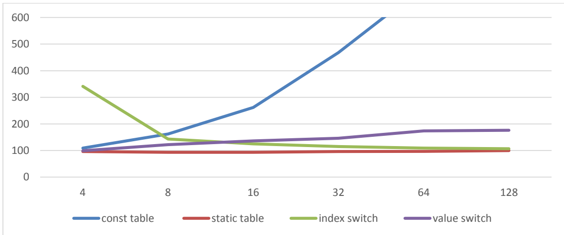
Graph 3.4.2: GCC 4.8.1 results
